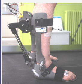
PAFO - Powered ankle-foot orthosis
